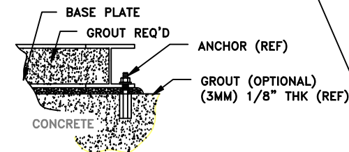
TYPICAL ANCHOR BOLT DETAIL FOR (25MM) 1.00 DIA, MOUNTING HOLE
